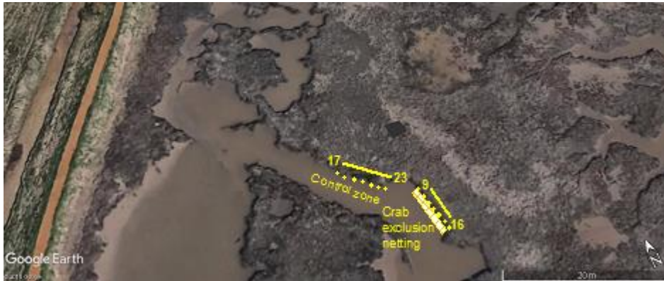
Figure 13a: Layout of measuring equipment north of Waldringfield
